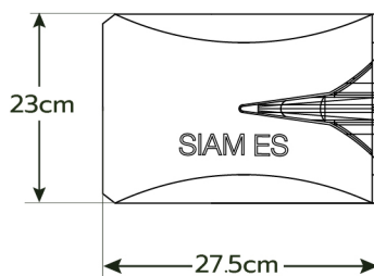
TOP VIEW Square Mouth Shovel
